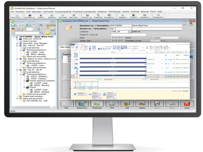
Radquote integration
