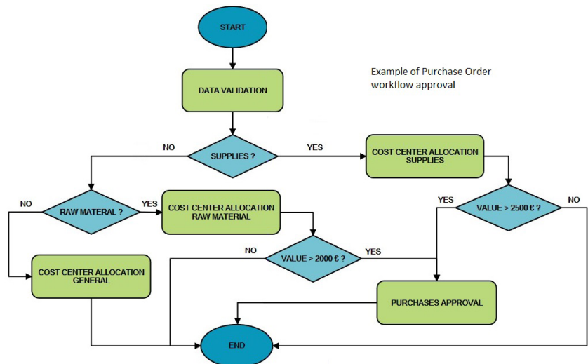
Workflow Module
